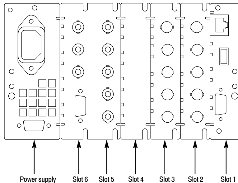
Figure G-1: WFM700 rear panel slot numbers (two input cards installed)
