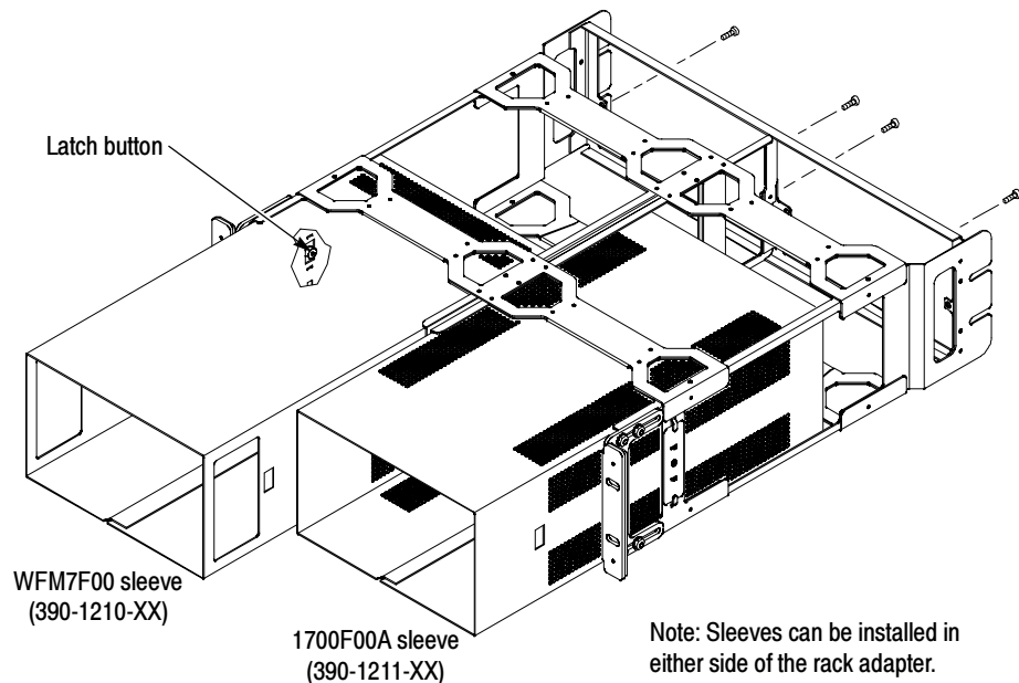
Figure F-14: Installing the sleeves into the WFM7F05 rack adapter
