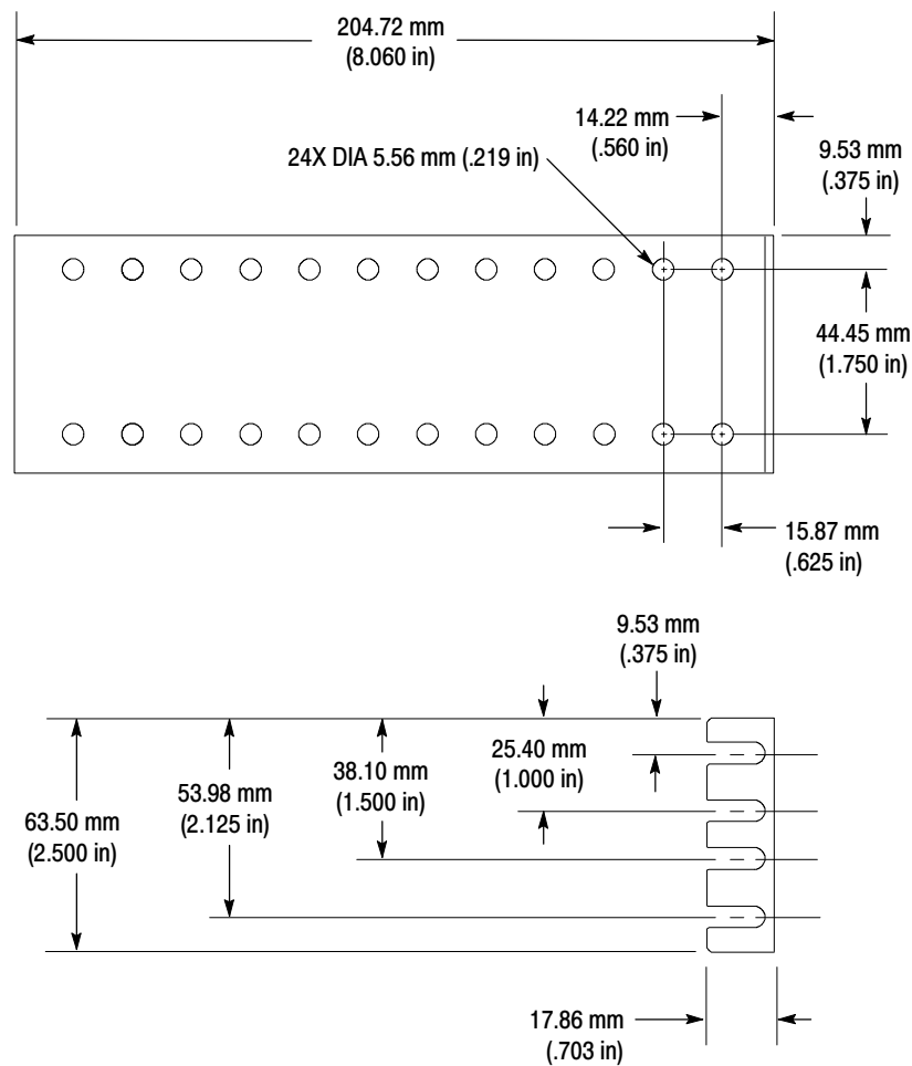
Figure F- 11: Rear bracket guide dimensions
