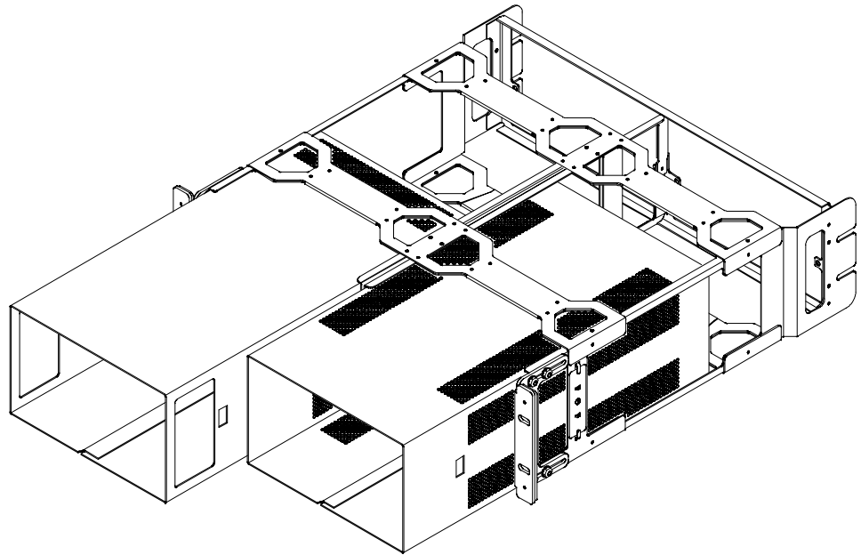
Figure 1-3: WFM7F05 Rack Adapter
