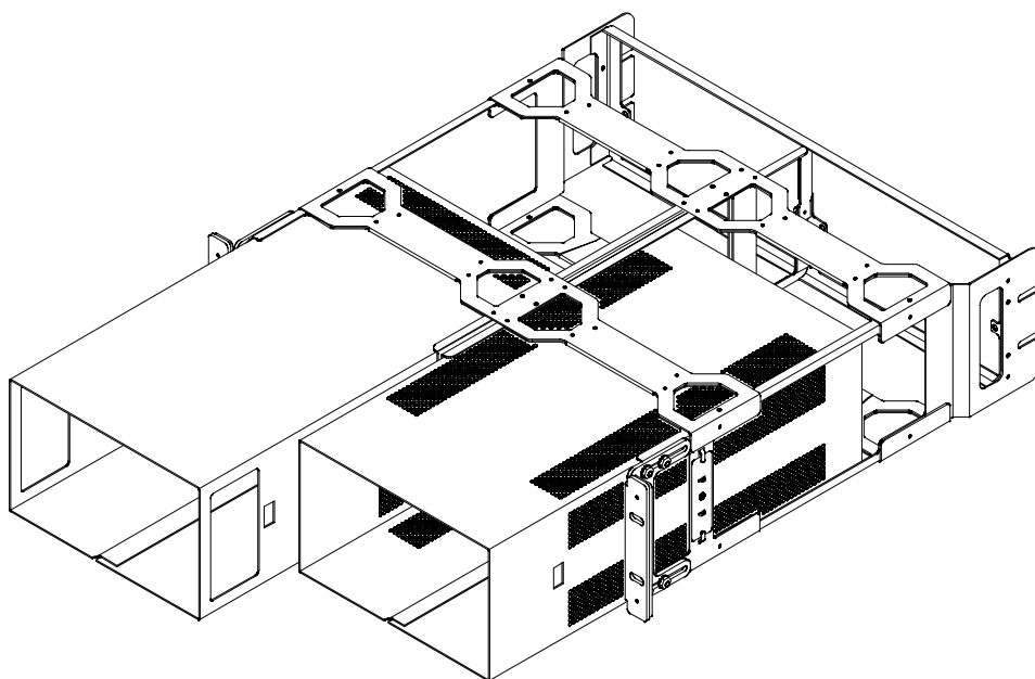
Figure F-8: WFM7F05 rack adapter
