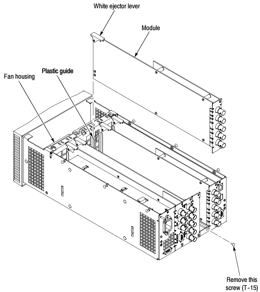
Figure G-3: Inserting the module into the chassis
