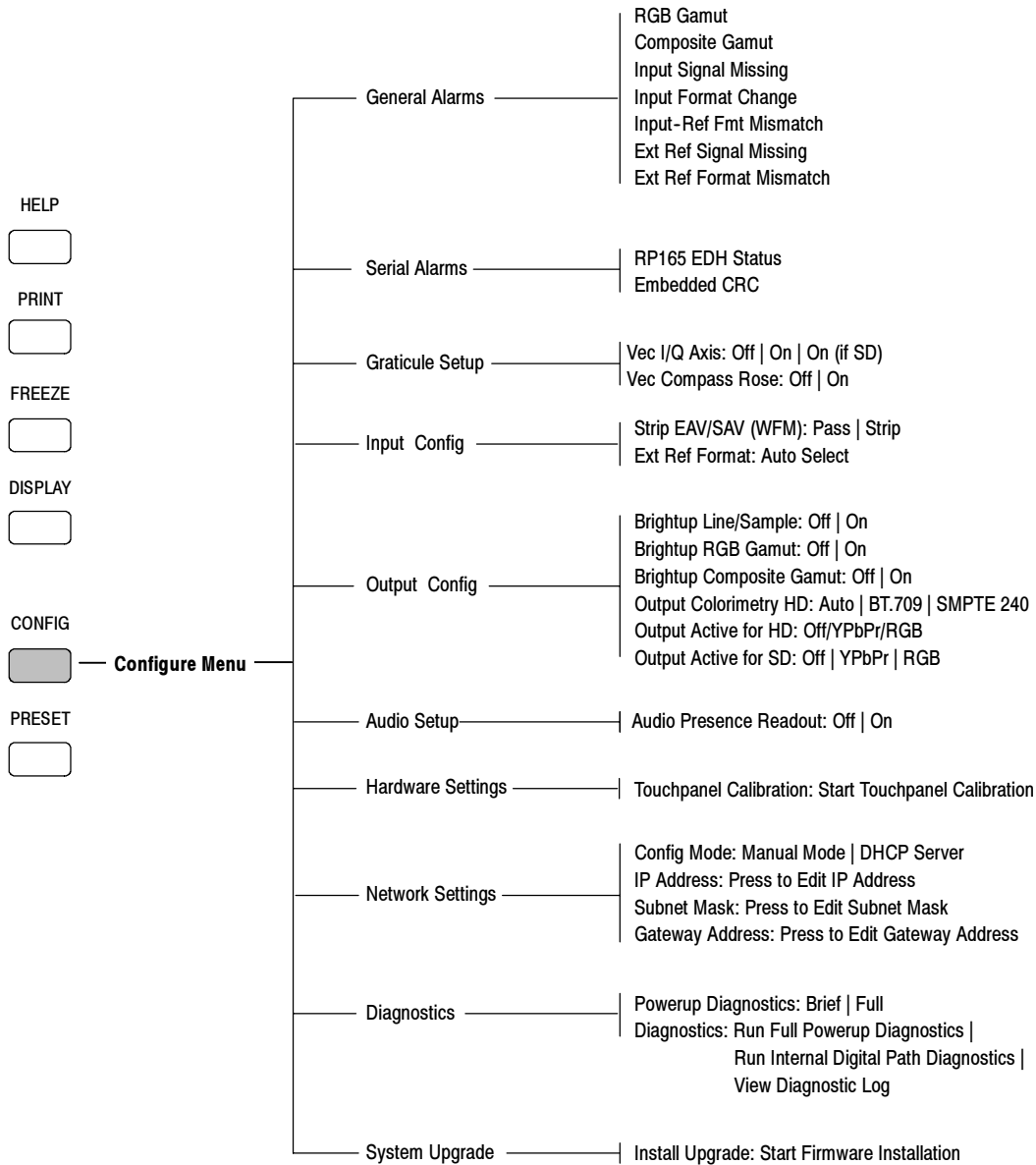
Figure 2-4: Configuration menu diagram
